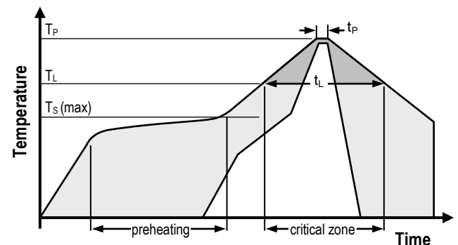
Figure 1 Soldering profile according to JEDEC standard. T_P \leq 260^\circ\text{C} and t_P \leq 30\text{sec} for Pb-free assembly. T_L < 220^\circ\text{C} and t_L < 150\text{sec} . Ramp-up/down speeds shall be < 5^\circ\text{C/sec} .
