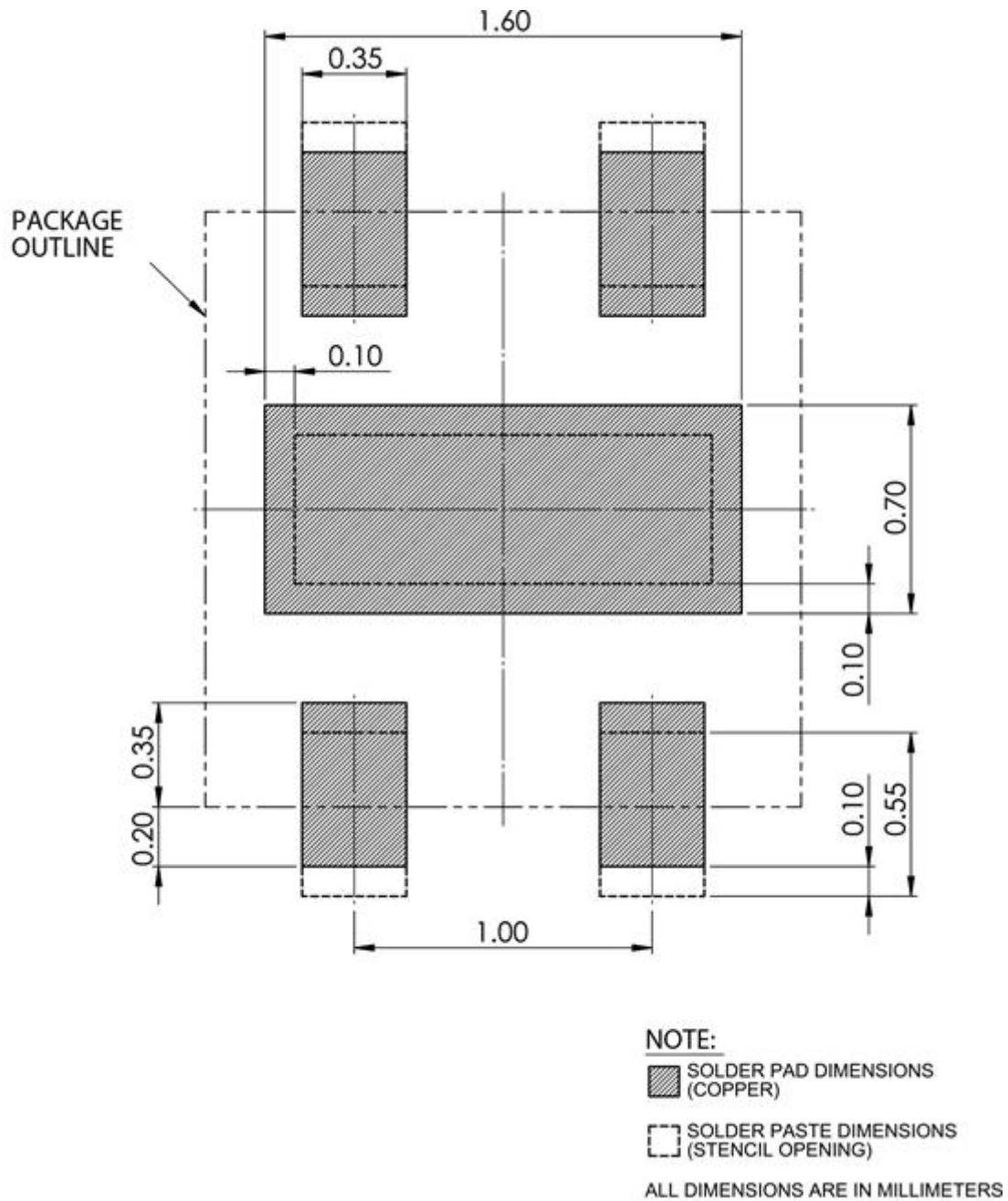
Figure 2 Recommended metal land pattern for SHTC1 (all dimensions are in mm). Recommended solder paste stencil thickness is 100µm, pads on PCB are recommended to be non solder mask defined (NSMD).
